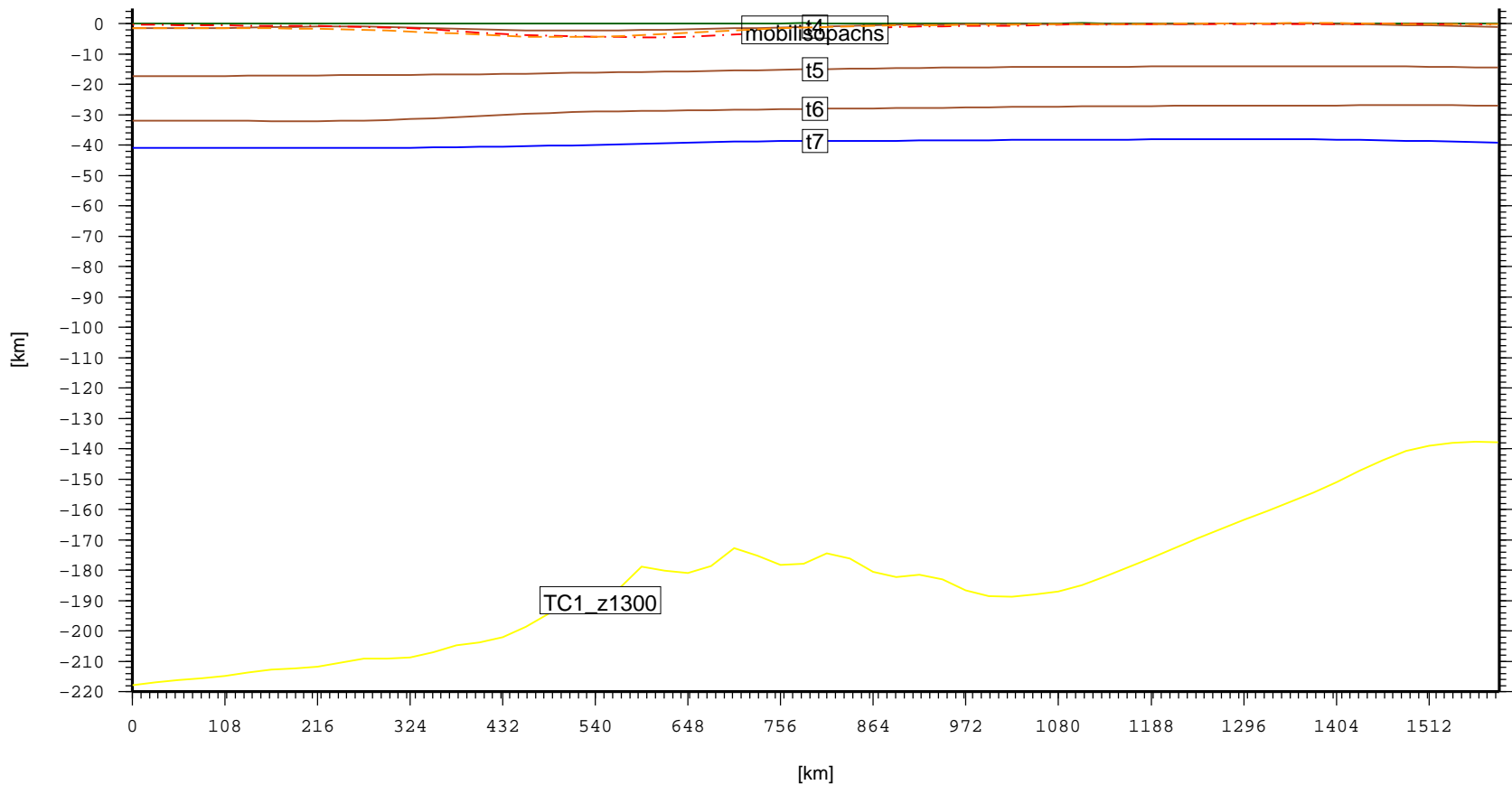
Cross section – SAM.AmazonasBasin (topo, laske sedthick, t4, t5, t6, t7)
