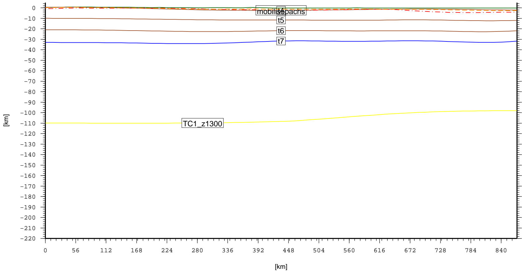
Cross section – SAM.AustralBasin (topo, laske sedthick, t4, t5, t6, t7)
