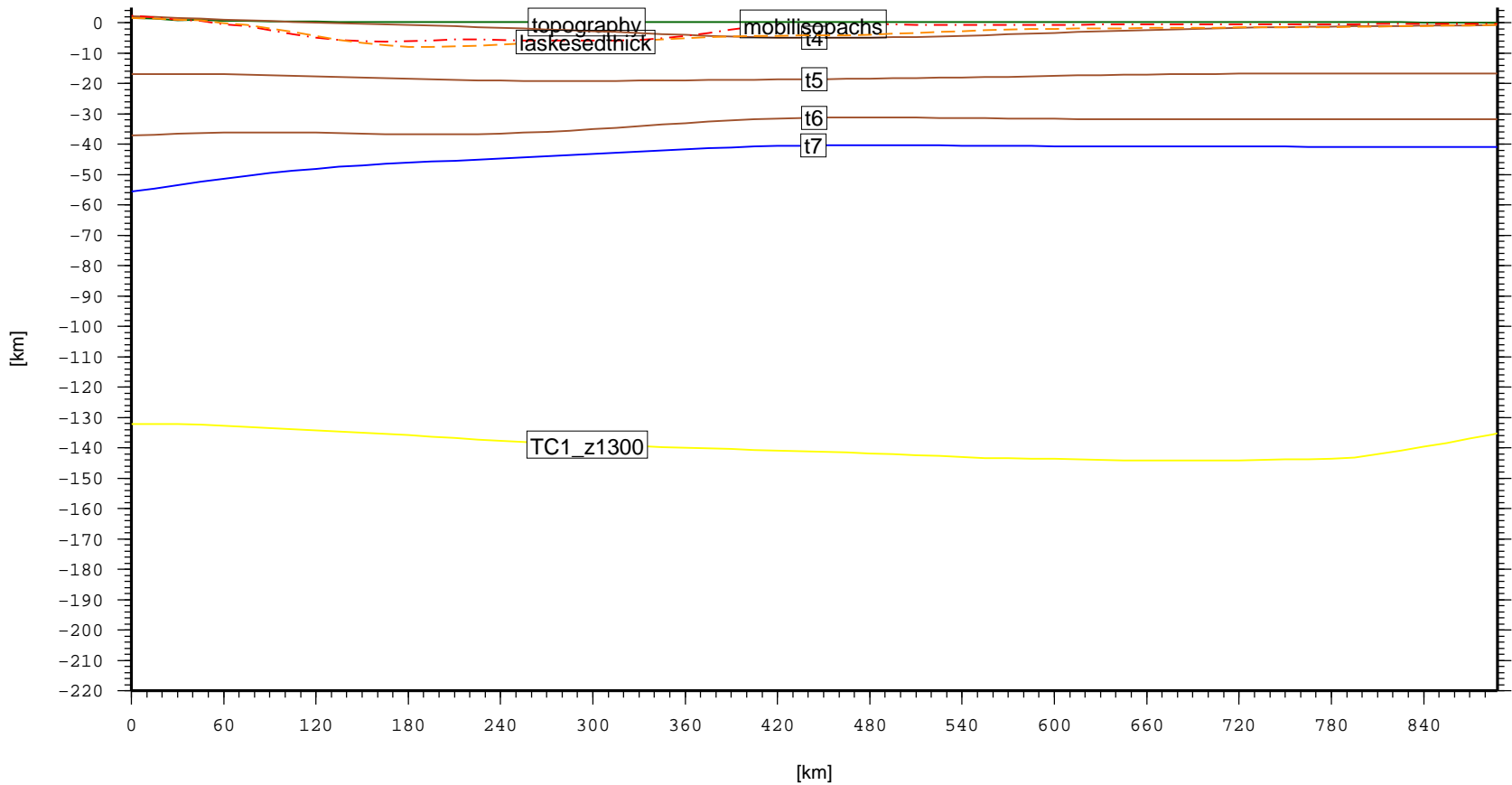
Cross section – SAM.ChacoBasin (topo, laske sedthick, t4, t5, t6, t7)
