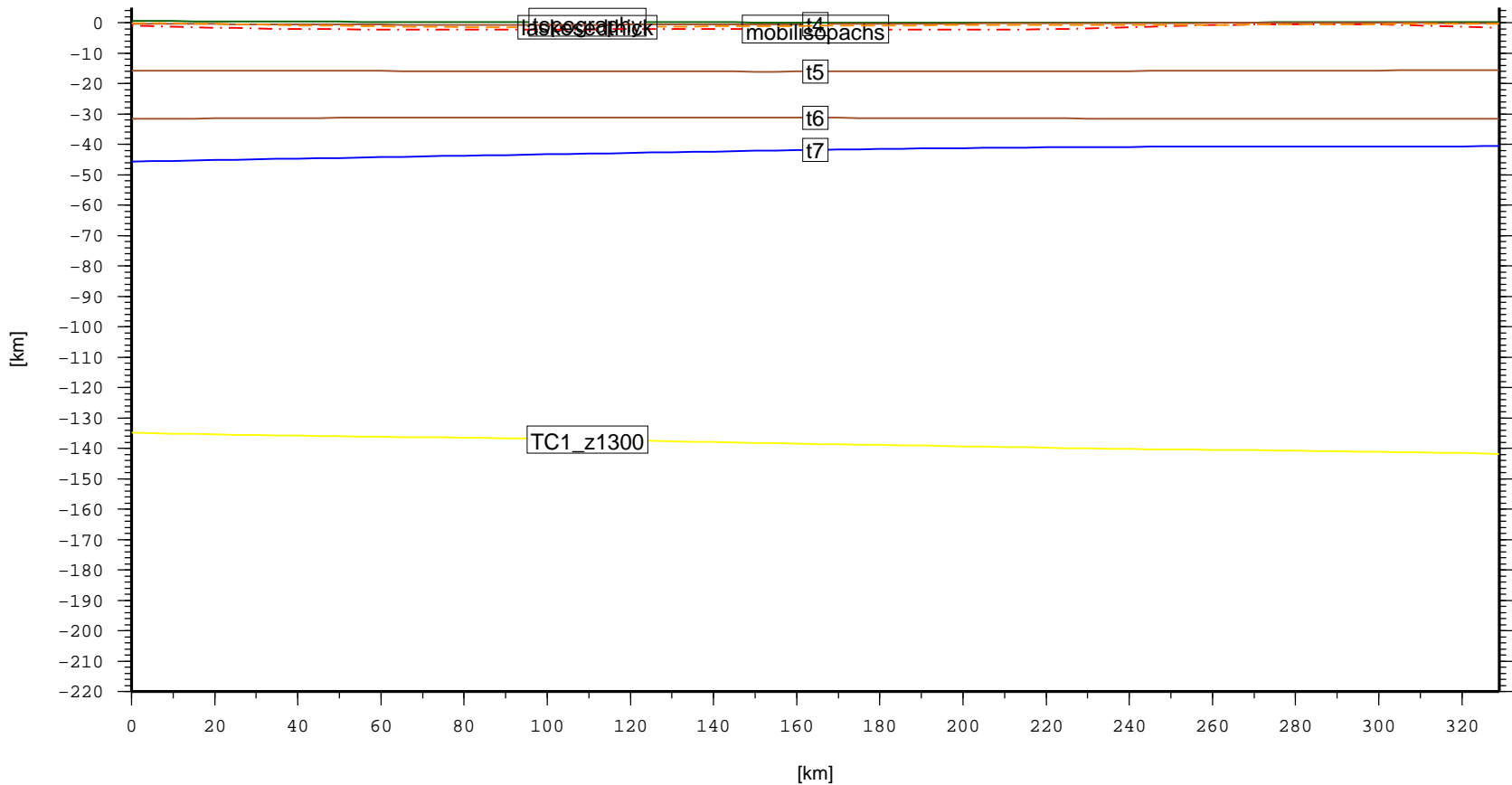
Cross section – SAM.LasSalinasBasin (topo, laske sedthick, t4, t5, t6, t7)
