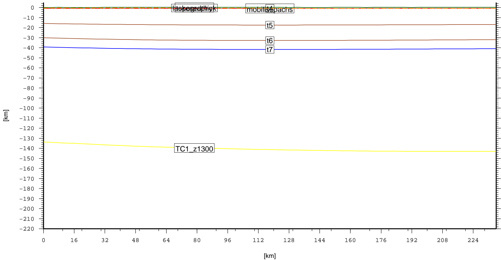
Cross section – SAM.MacachinBasin (topo, laske sedthick, t4, t5, t6, t7)
