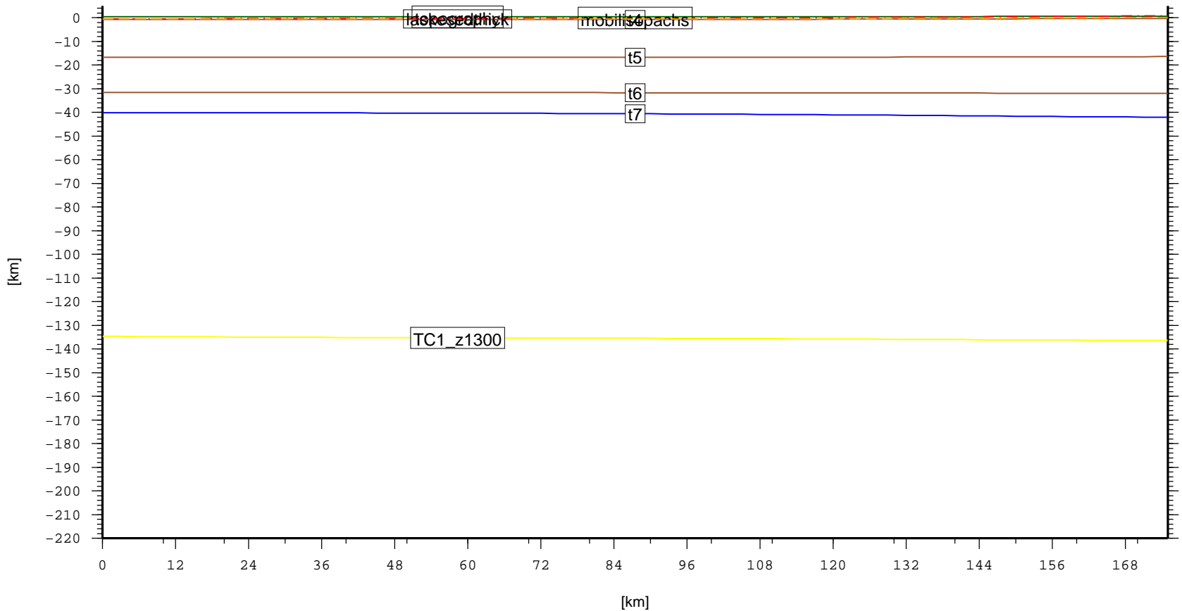
Cross section – SAM.MercedesBasin (topo, laske sedthick, t4, t5, t6, t7)
