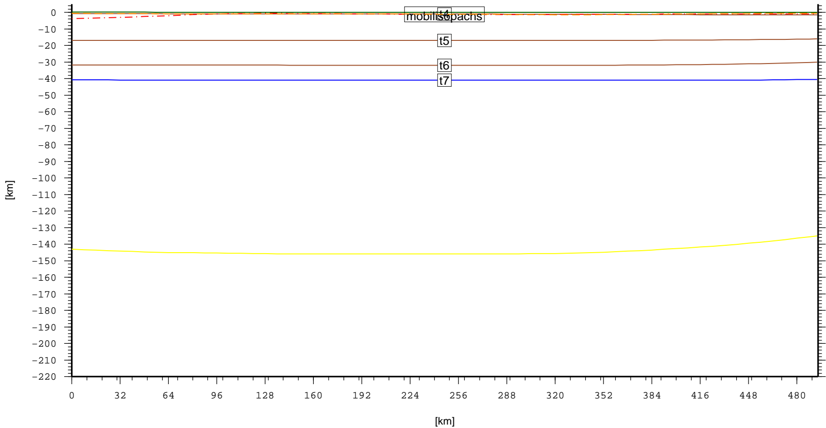
Cross section – SAM.RosarioBasin (topo, laske sedthick, t4, t5, t6, t7)
