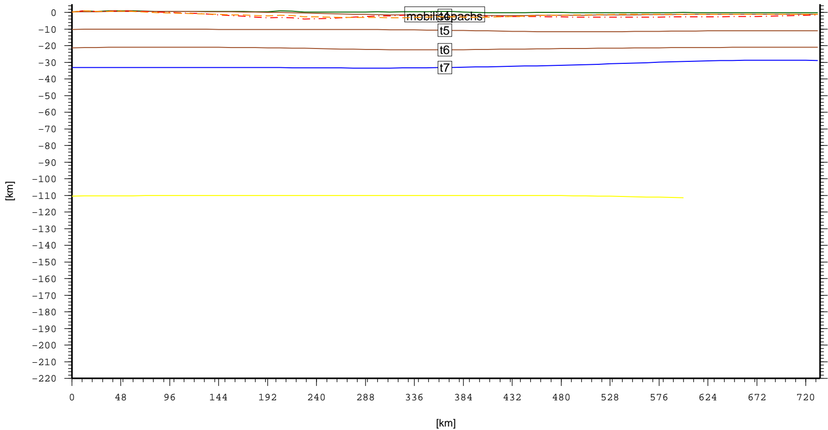
Cross section – SAM.SanJorgeBasin (topo, laske sedthick, t4, t5, t6, t7)
