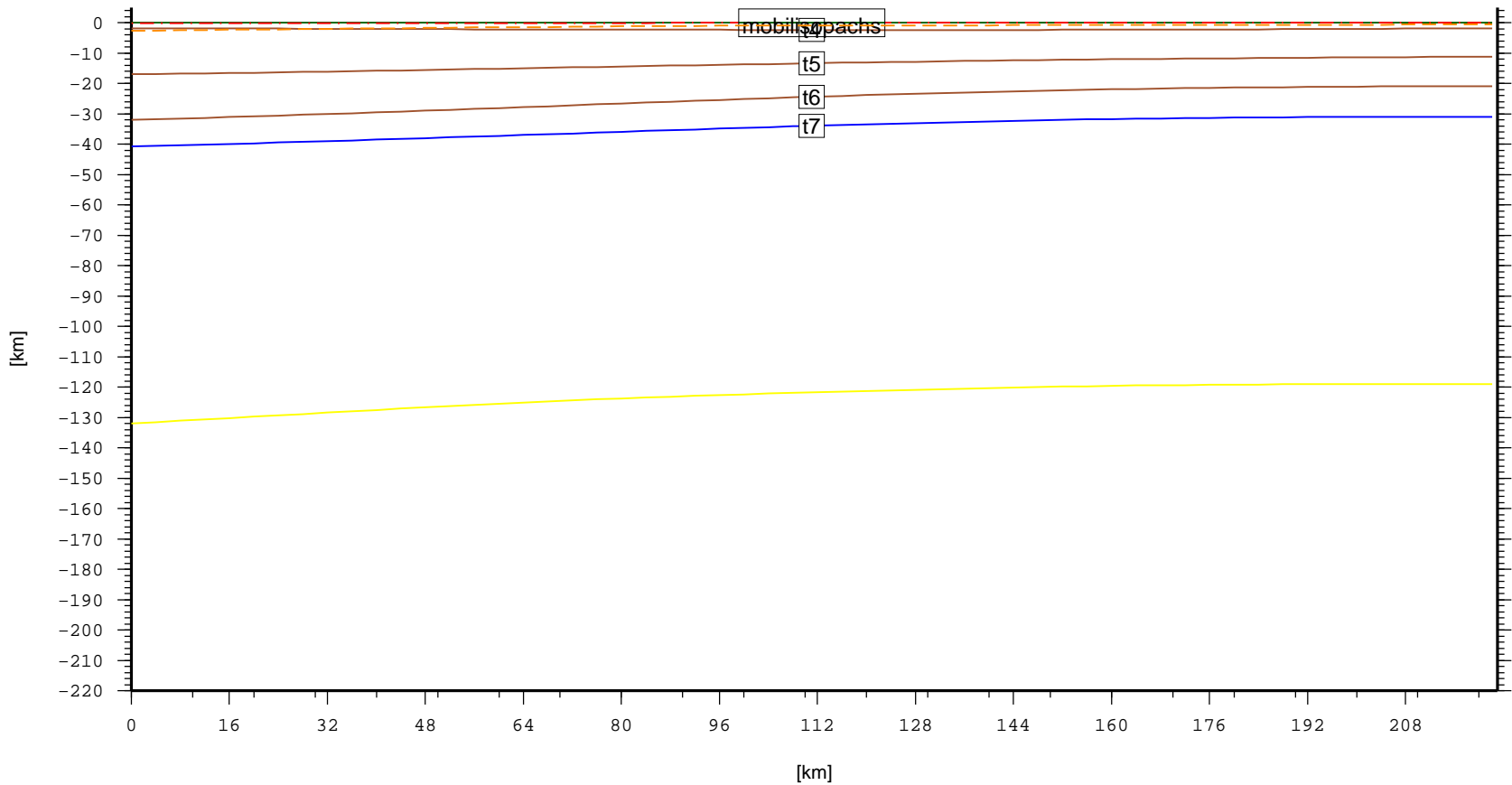
Cross section – SAM.SantaLuciaBasin (topo, laske sedthick, t4, t5, t6, t7)
