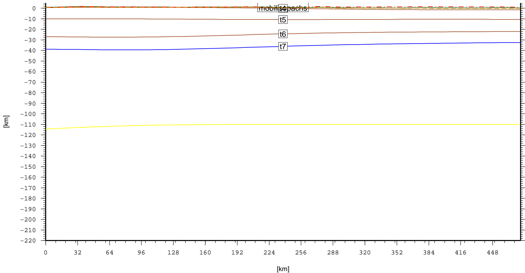
Cross section – SAM.Somuncura–CanadonAsfaltoBasin (topo, laske sedthick, t4, t5, t6, t7)
