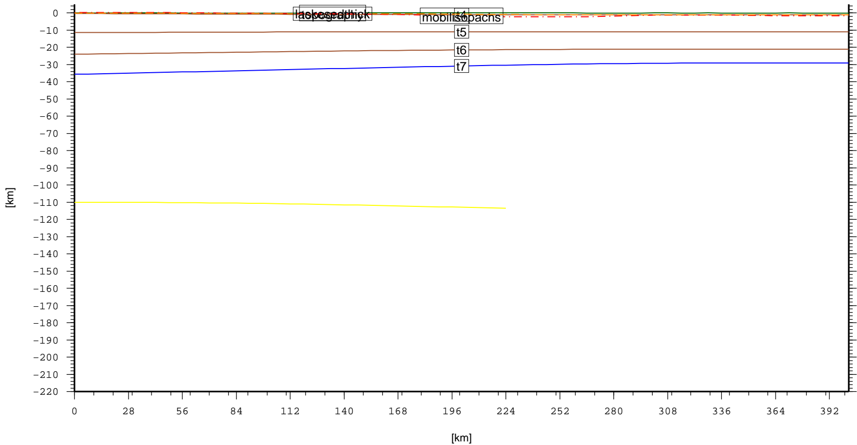
Cross section – SAM.ValdesBasin (topo, laske sedthick, t4, t5, t6, t7)
