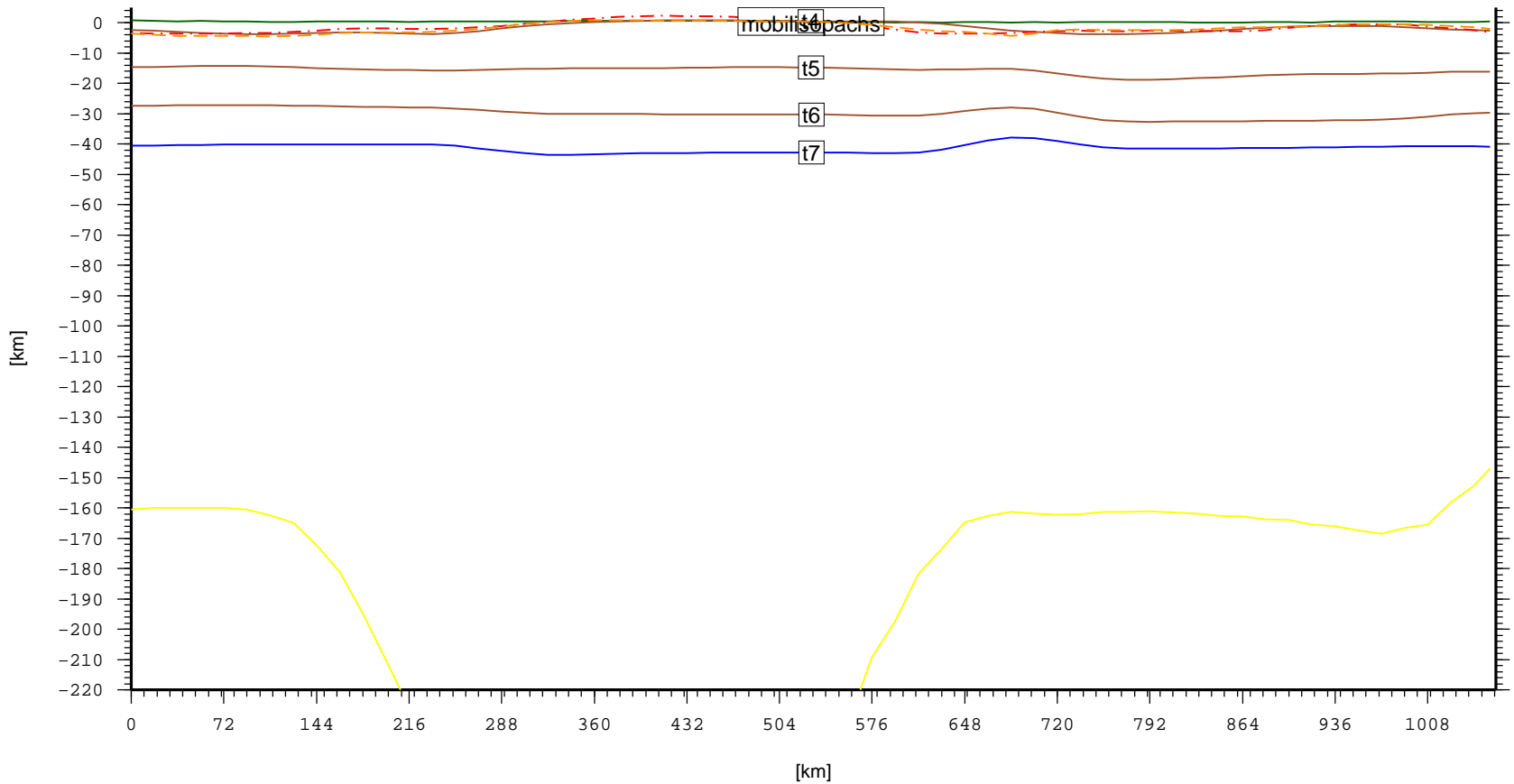
Cross section – SIB.Anabar–OlenekBasin (topo, laske sedthick, t4, t5, t6, t7)
