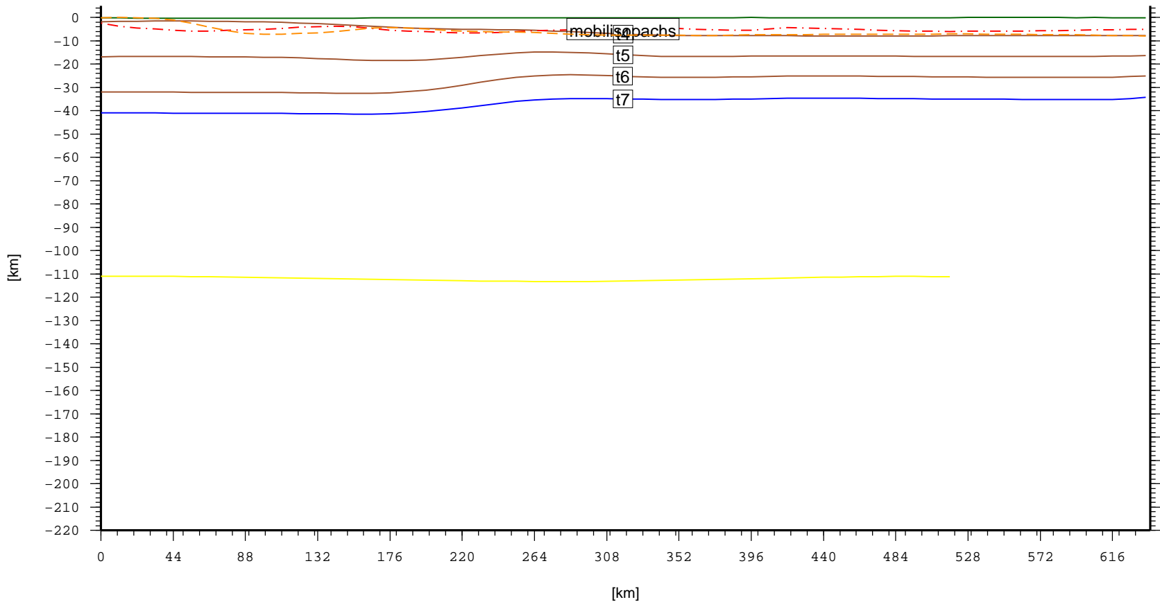
Cross section – SIB.EastNovayaZemlyaTrough (topo, laske sedthick, t4, t5, t6, t7)
