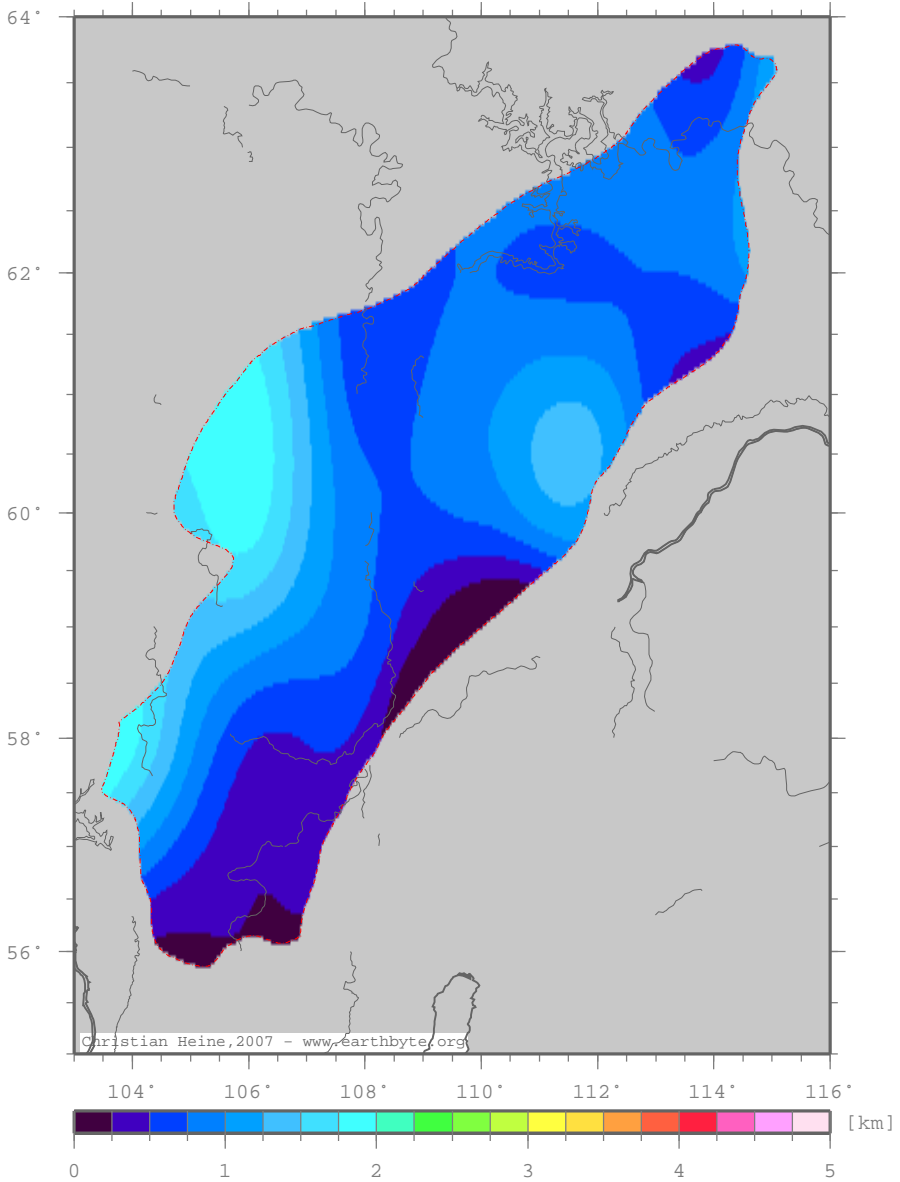
Total tectonic subsidence
