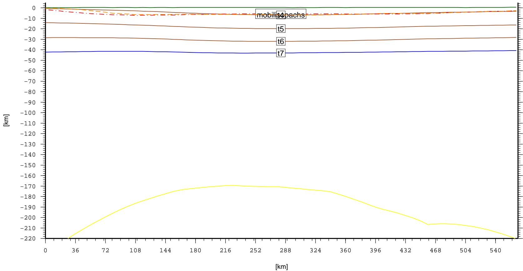
Cross section – SIB.Prisayan–YeniseySyncline (topo, laske sedthick, t4, t5, t6, t7)
