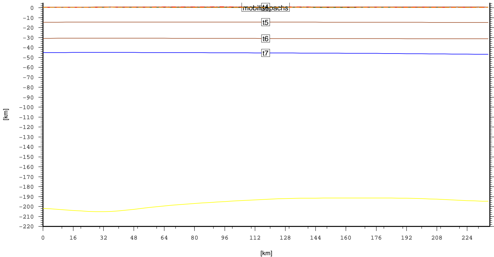
Cross section – SIB.RybinskayaDepression (topo, laske sedthick, t4, t5, t6, t7)
