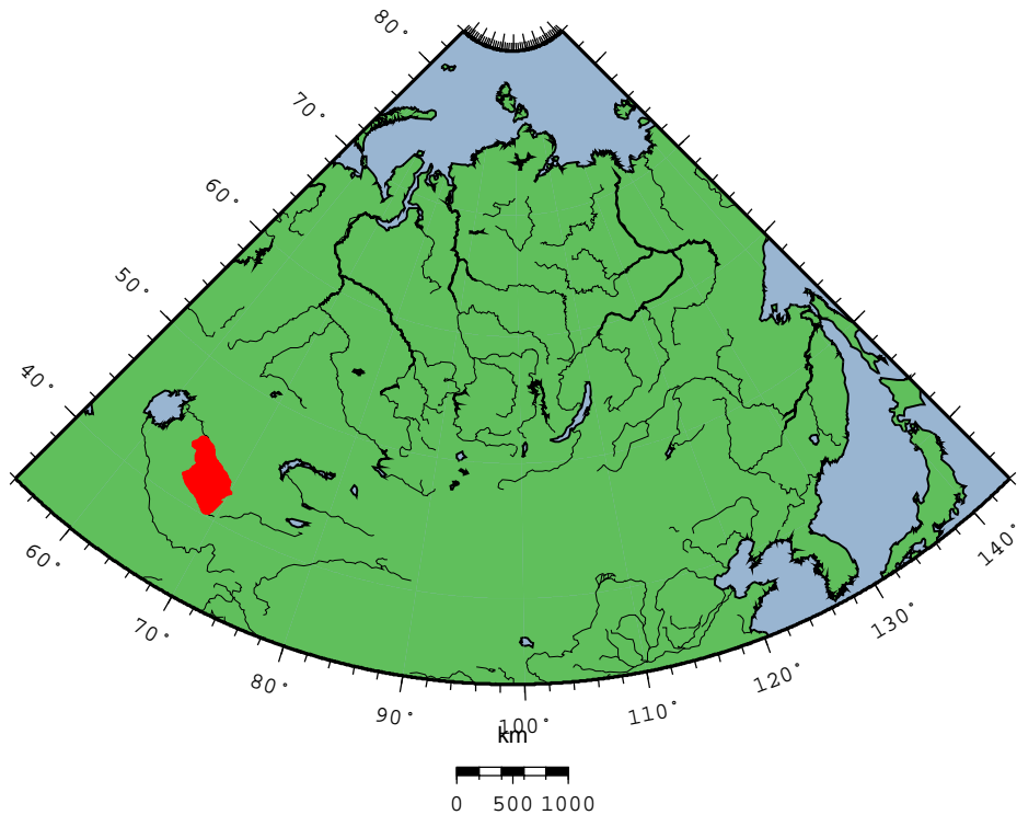
Location map SIB.Syr–DaryaBasin.
