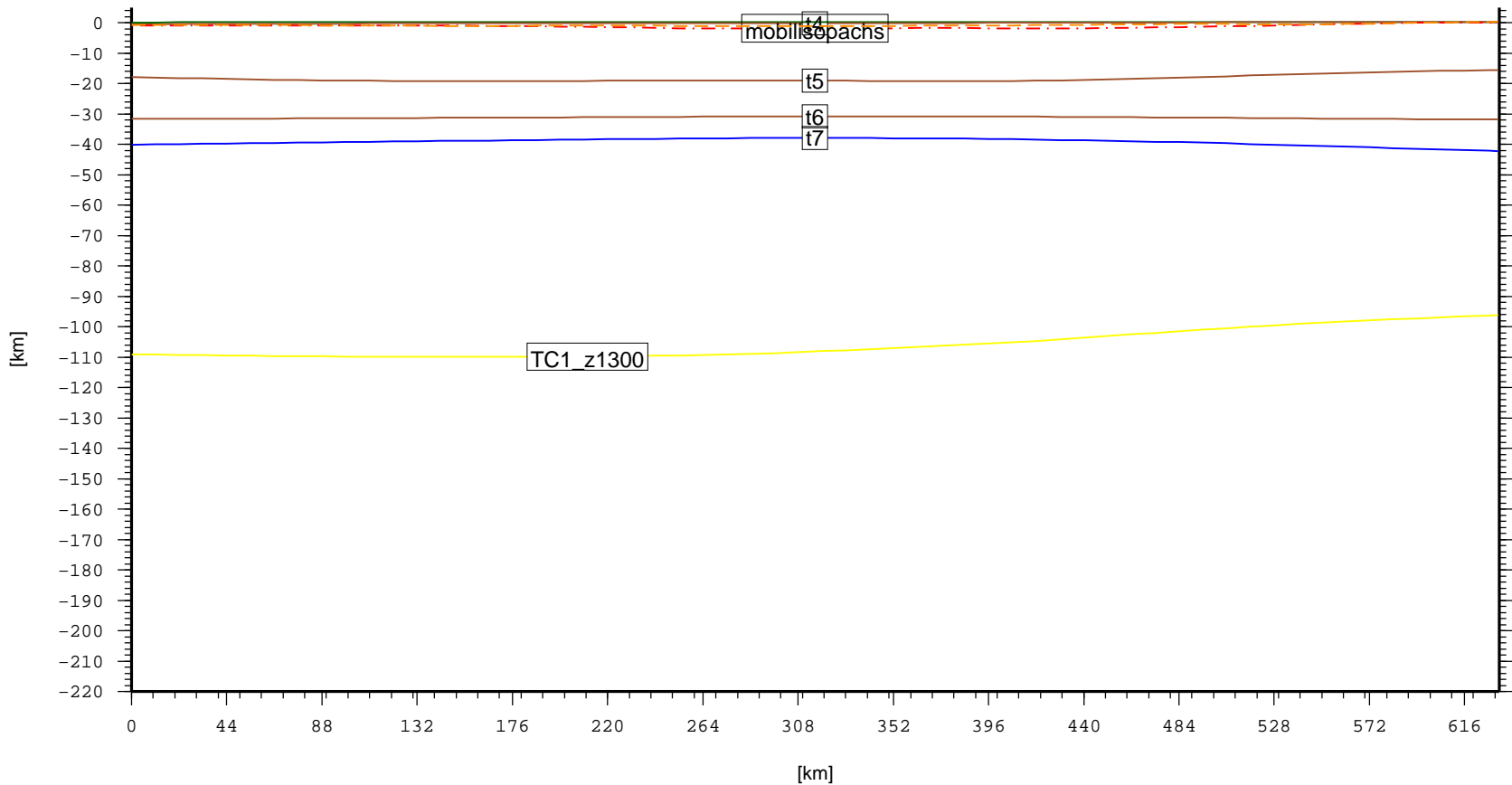
Cross section – SIB.Syr–DaryaBasin (topo, laske sedthick, t4, t5, t6, t7)
