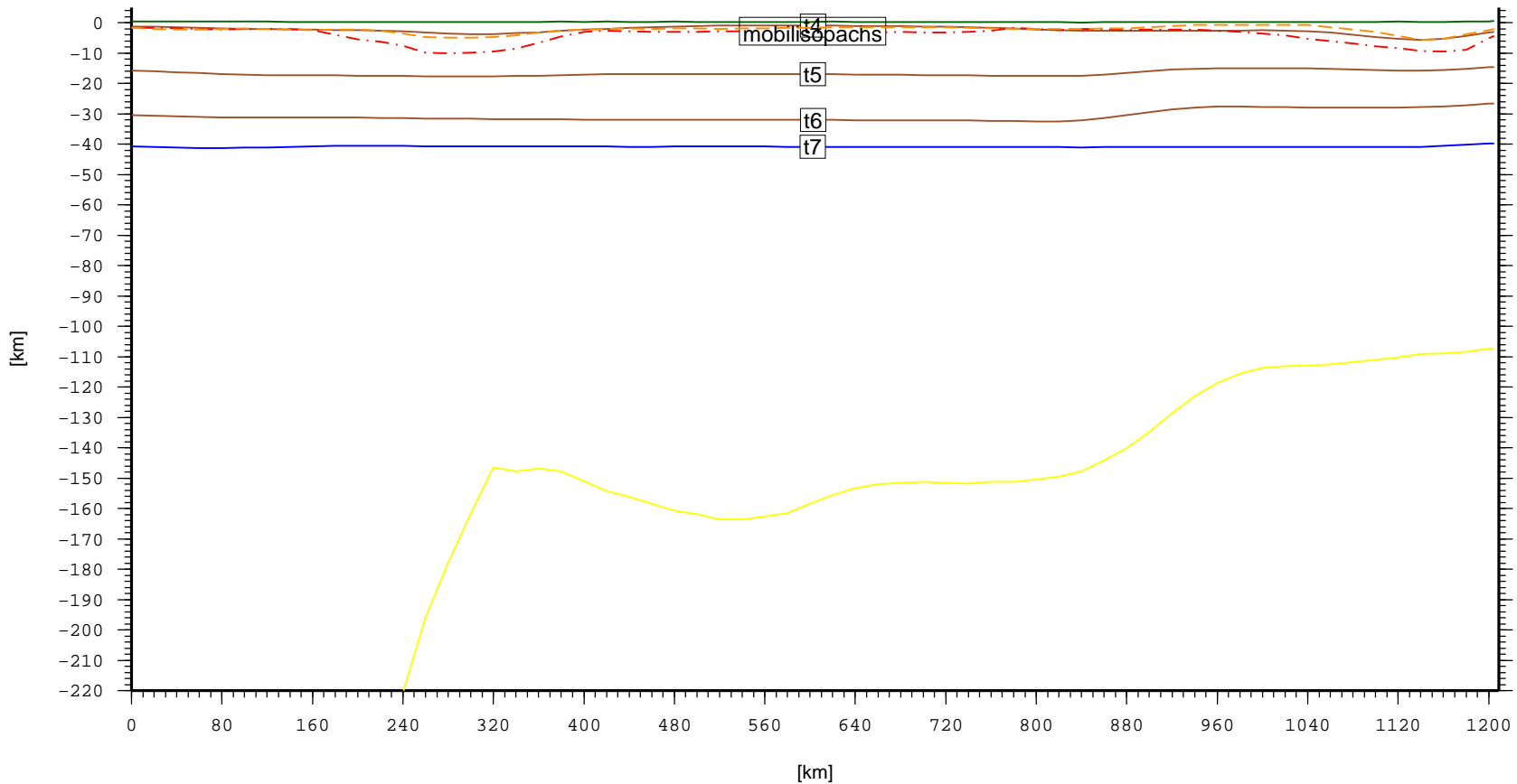
Cross section – SIB.VilyuyBasin (topo, laske sedthick, t4, t5, t6, t7)
