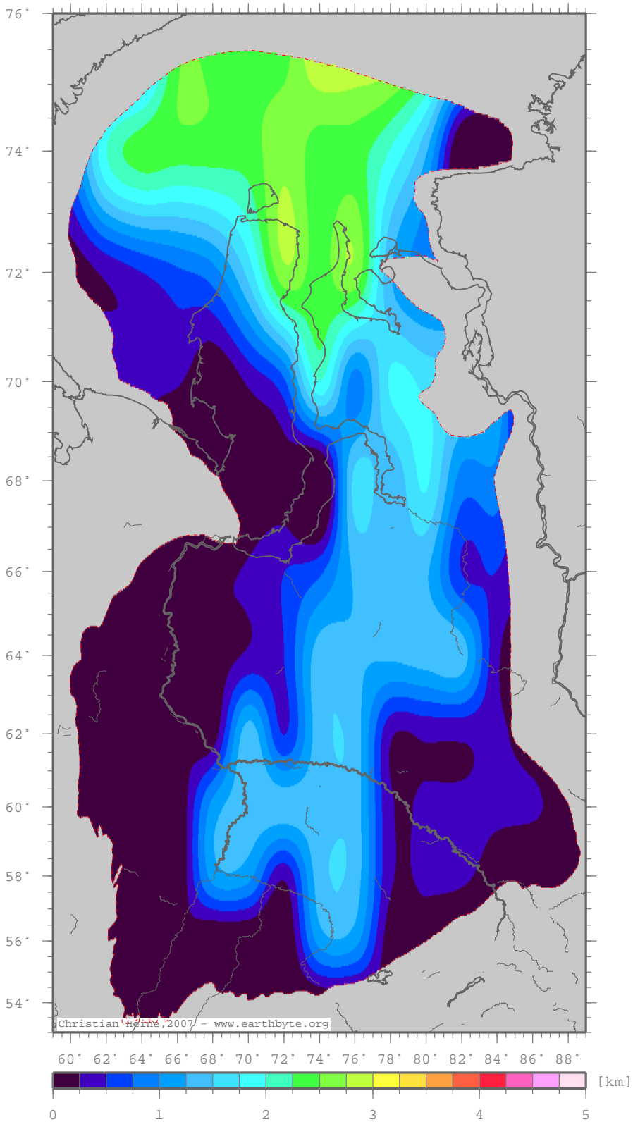
Total tectonic subsidence
