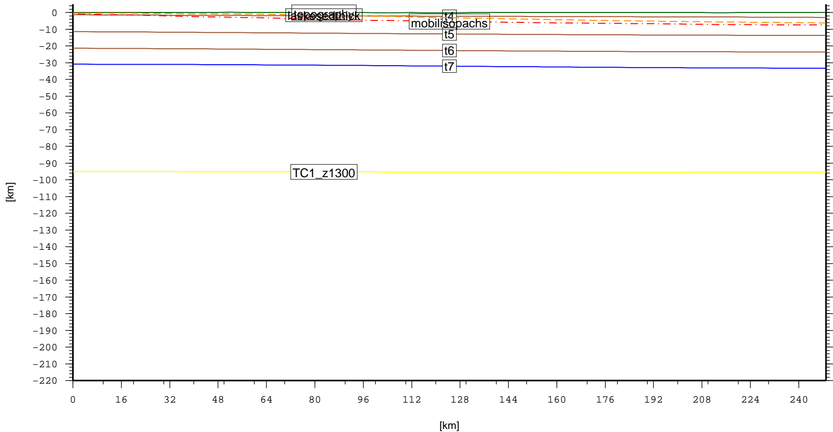
Cross section – SUN.BalingianProvince (topo, laske sedthick, t4, t5, t6, t7)
