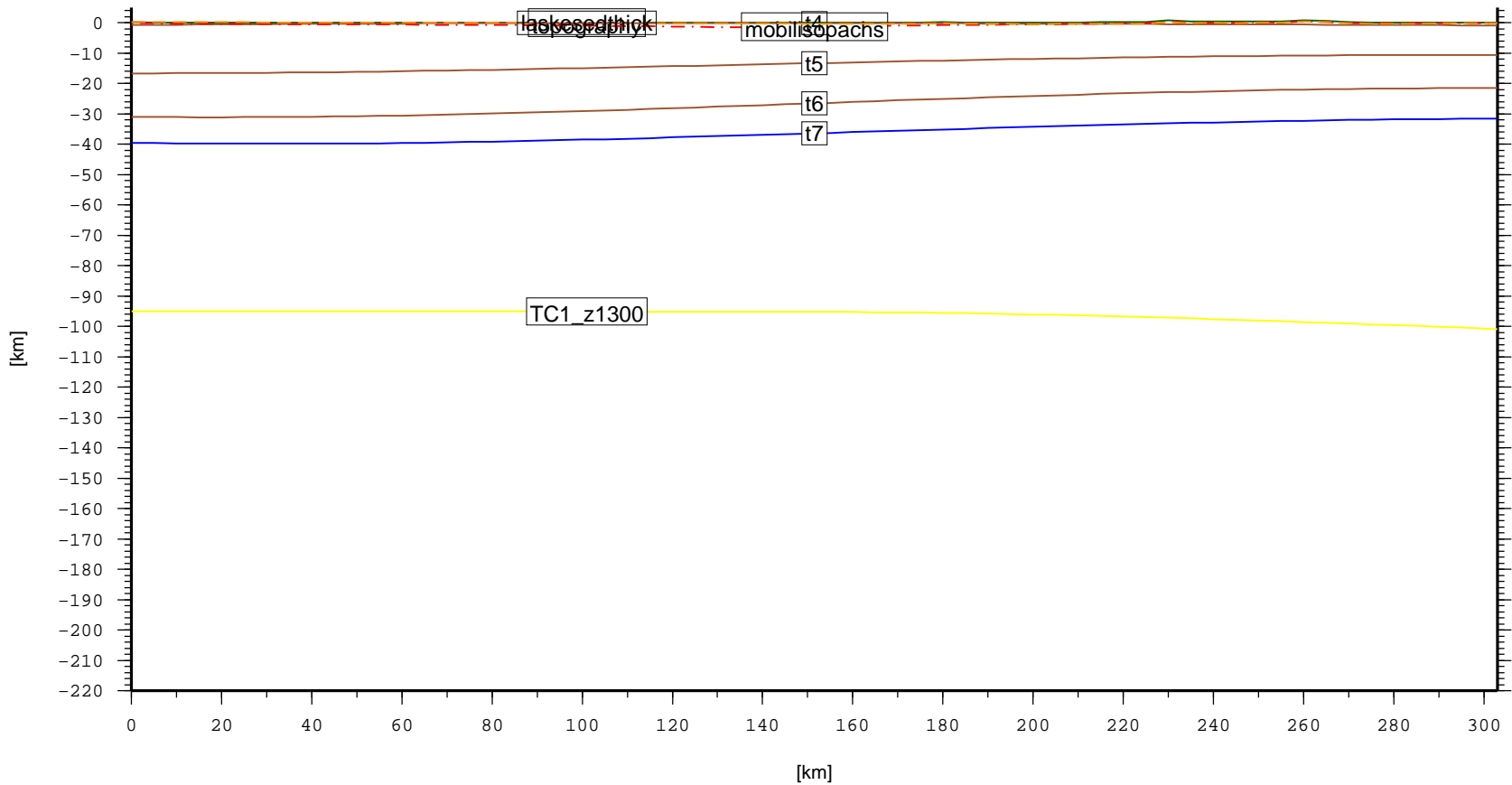
Cross section – SUN.ChaoPhrayaBasin (topo, laske sedthick, t4, t5, t6, t7)
