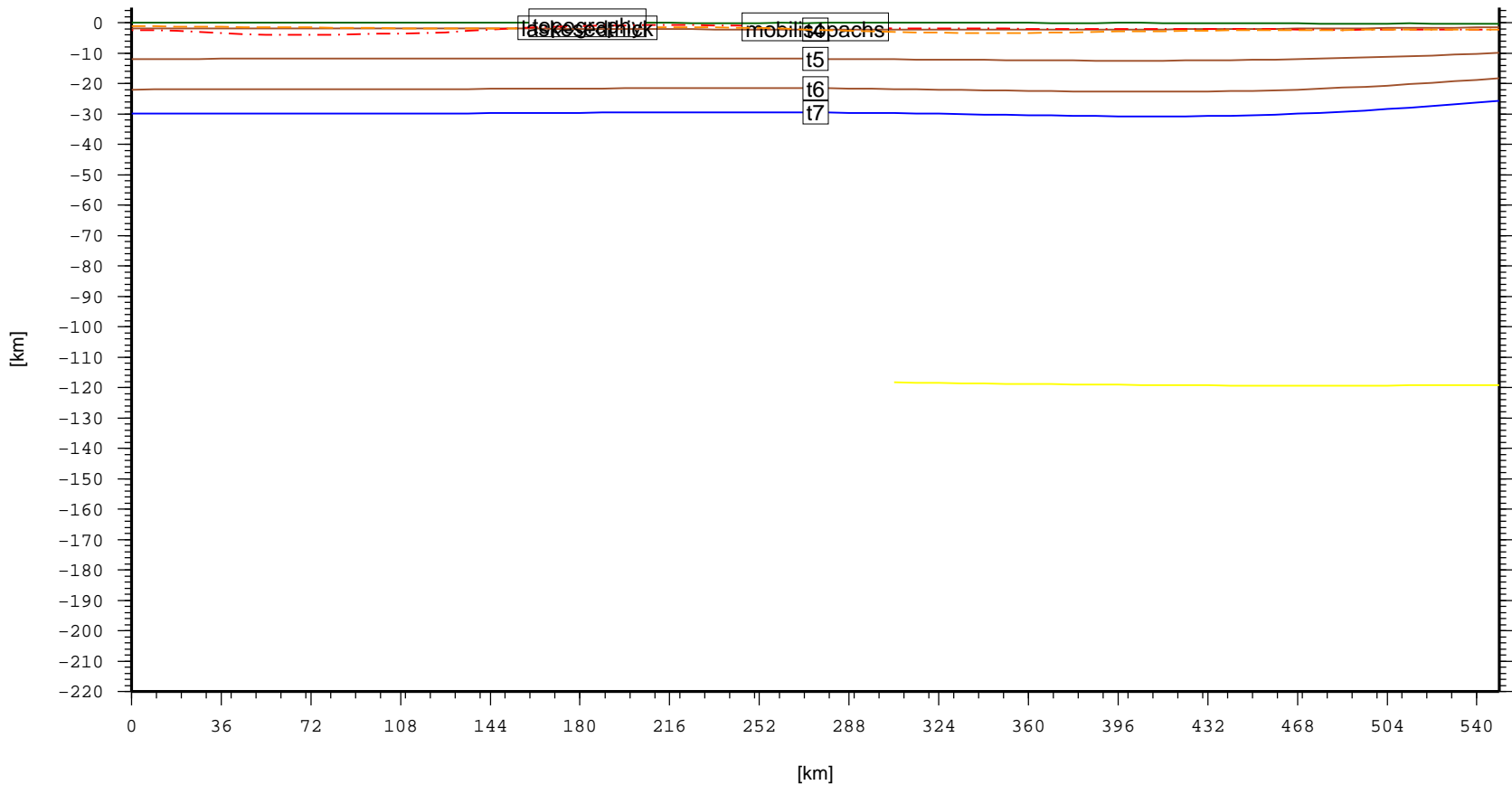
Cross section – SUN.ConSonSwell (topo, laske sedthick, t4, t5, t6, t7)
