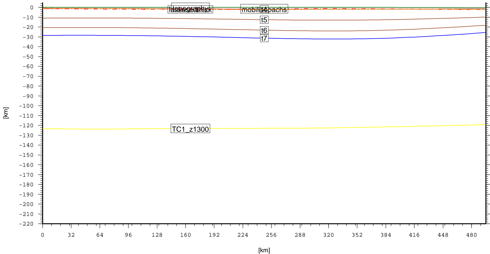
Cross section – SUN.CuuLongBasin (topo, laske sedthick, t4, t5, t6, t7)
