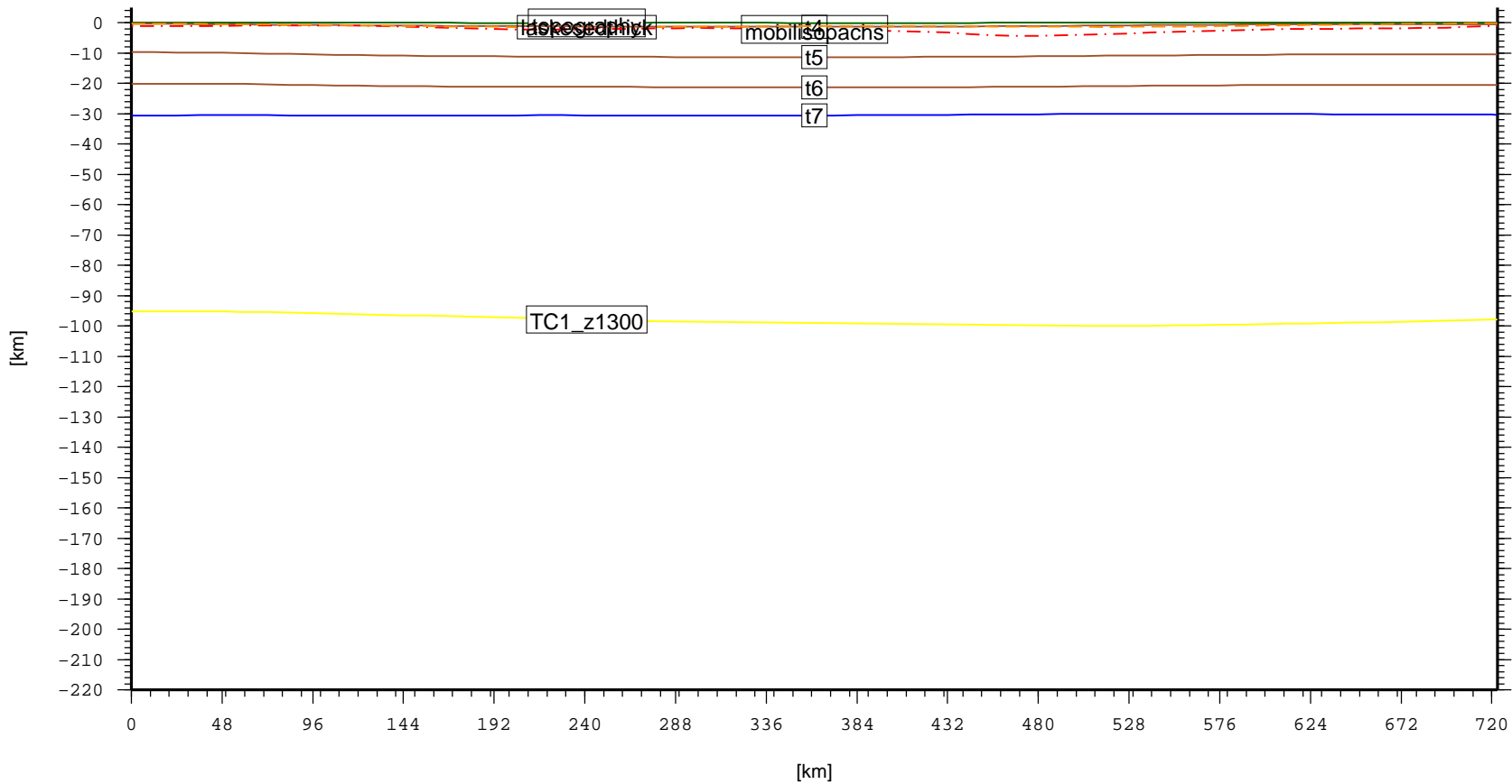
Cross section – SUN.GulfofThailandBasin (topo, laske sedthick, t4, t5, t6, t7)
