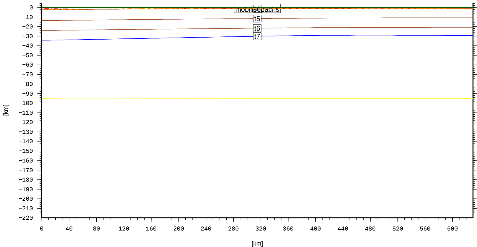
Cross section – SUN.KarimunjawaArch (topo, laske sedthick, t4, t5, t6, t7)
