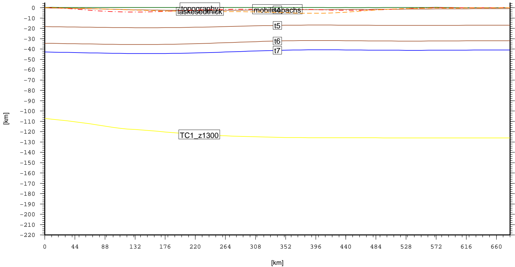
Cross section – SUN.KhoratPlateauBasin (topo, laske sedthick, t4, t5, t6, t7)
