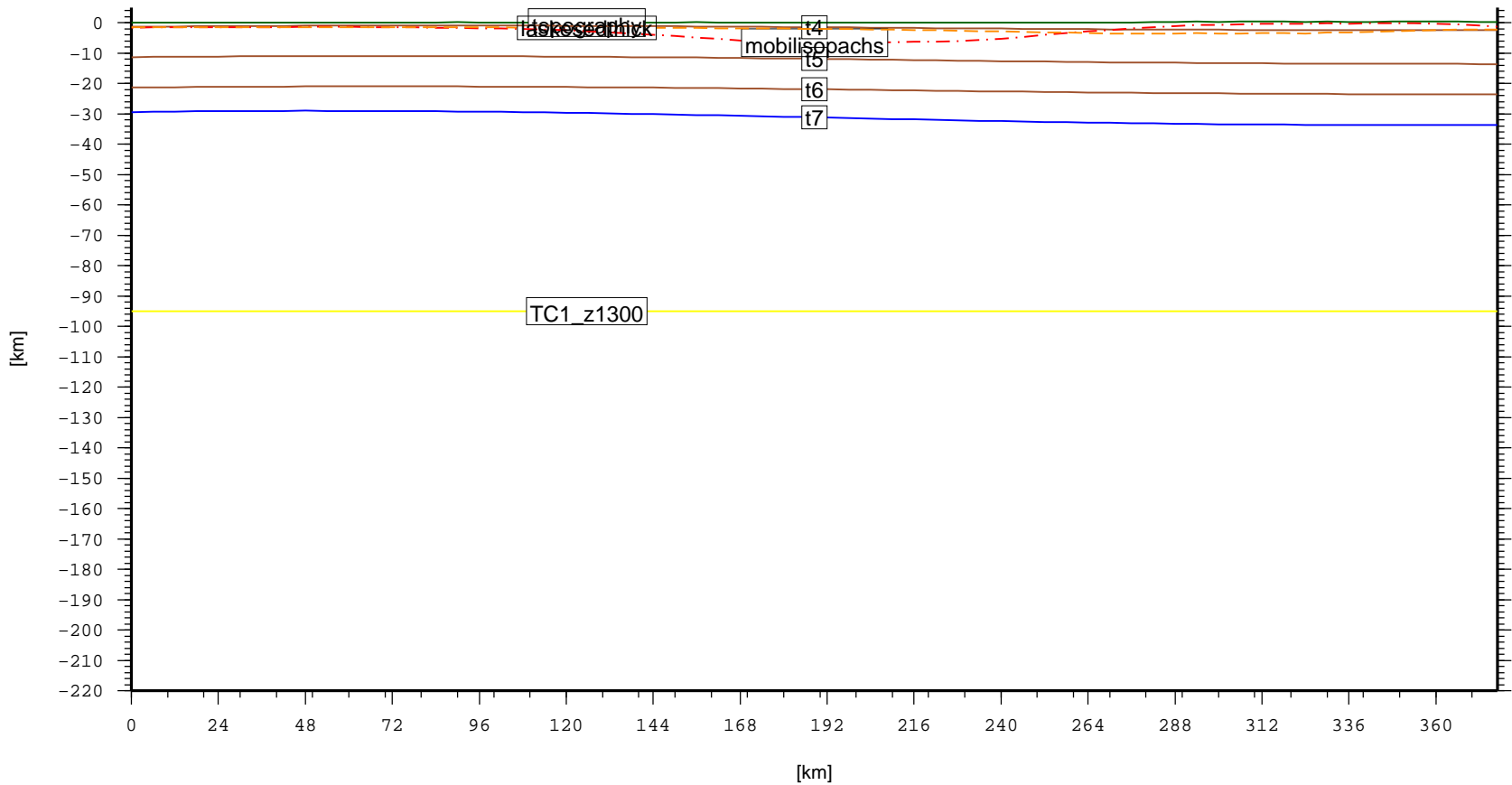
Cross section – SUN.MeratusHigh (topo, laske sedthick, t4, t5, t6, t7)
