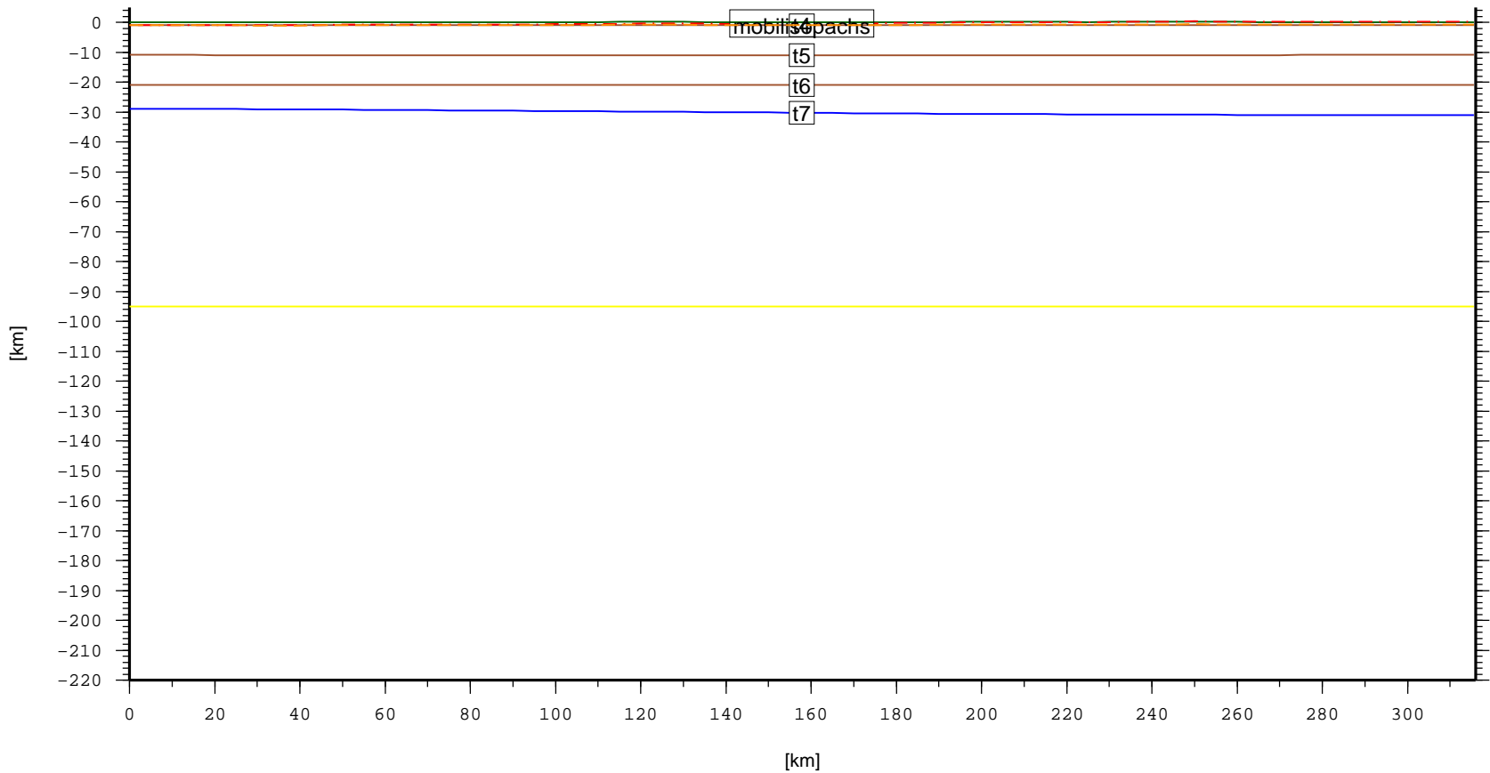
Cross section – SUN.PembuangBasin (topo, laske sedthick, t4, t5, t6, t7)
