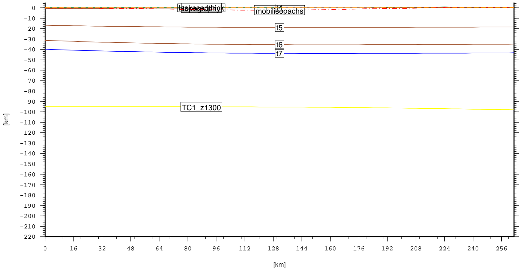
Cross section – SUN.PhitsanulokBasin (topo, laske sedthick, t4, t5, t6, t7)
