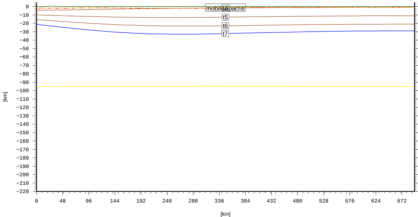
Cross section – SUN.WestJavaBasin (topo, laske sedthick, t4, t5, t6, t7)
