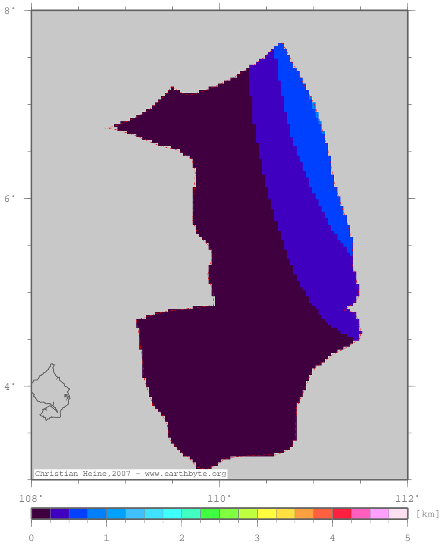
Total tectonic subsidence
