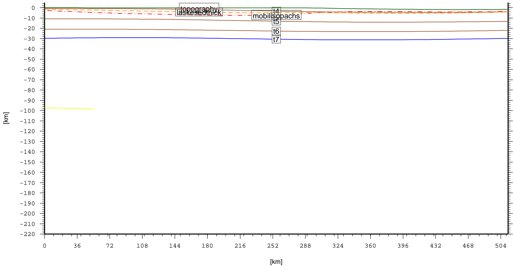
Cross section – SUN.WestLuconiaProvince (topo, laske sedthick, t4, t5, t6, t7)
