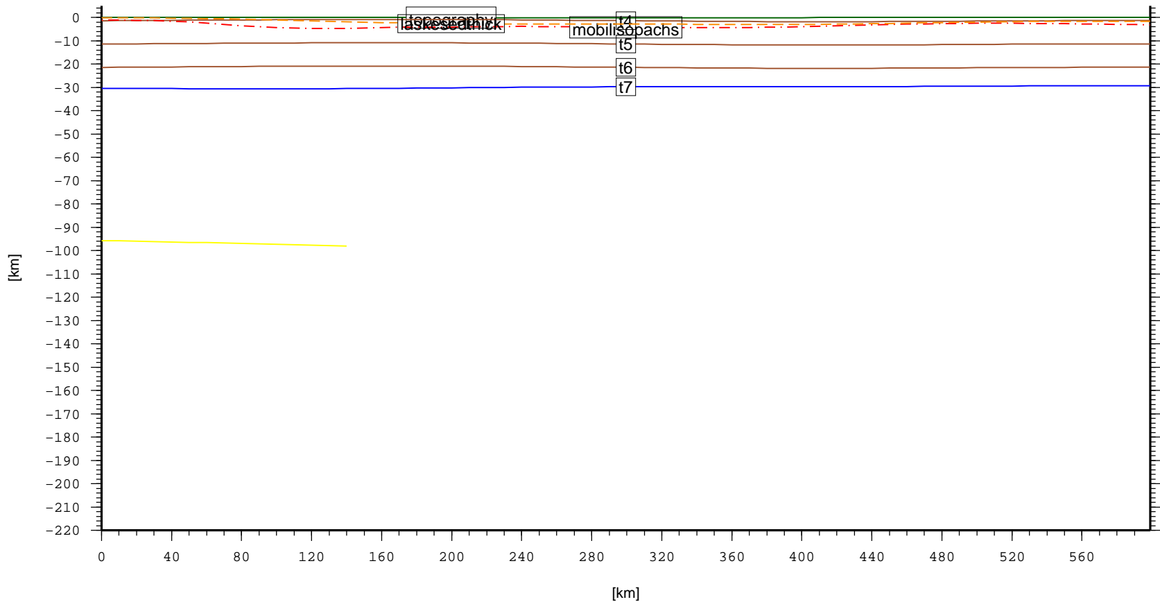
Cross section – SUN.WestNatunaBasin (topo, laske sedthick, t4, t5, t6, t7)
