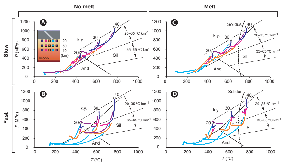
Figure 3. Pressure, temperature, time ( P-T-t ) paths in migmatite-cored metamorphic core complexes for slow and fast strain rates in no-melt models (A, B) and melt-present models (C, D). Color of P-T-t paths refers to markers shown in inset in A; their original depths are 20, 30, and 40 km.
