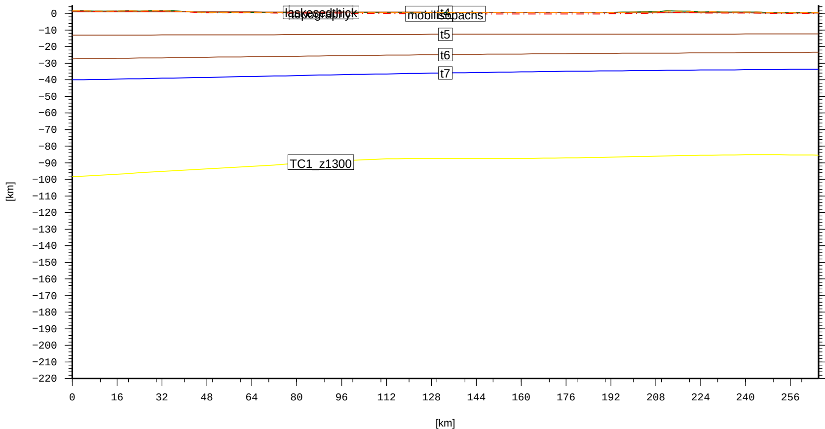
Cross section – AFR.LotikipiBasin (topo, laske sedthick, t4, t5, t6, t7)
