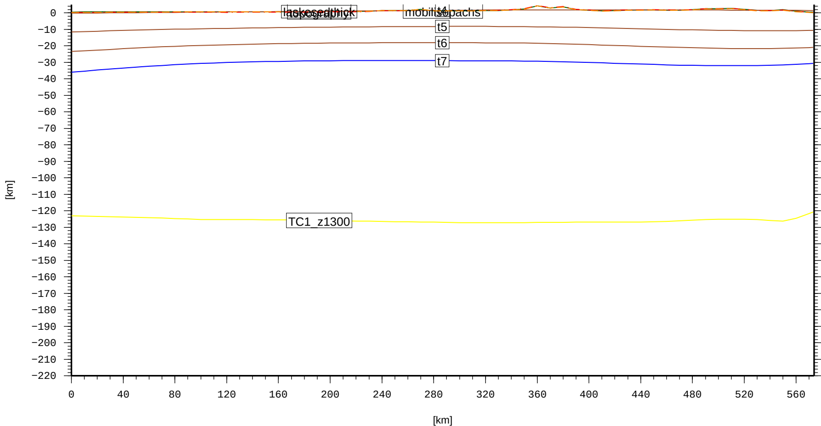
Cross section – AFR.MekeleBasin (topo, laske sedthick, t4, t5, t6, t7)
