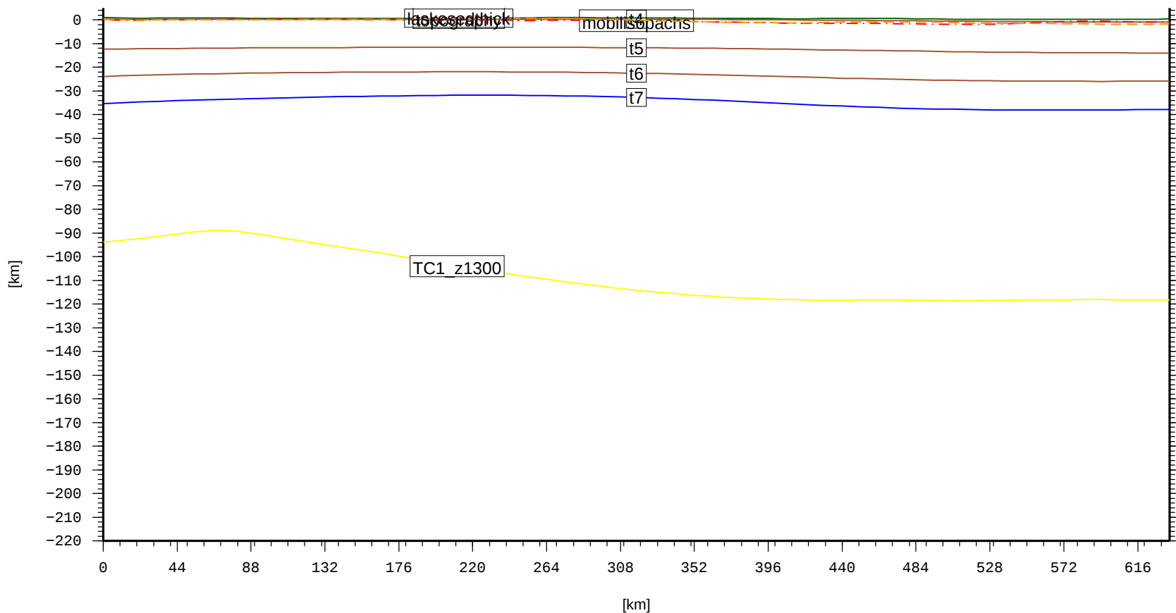
Cross section – AFR.SelousBasin (topo, laske sedthick, t4, t5, t6, t7)
