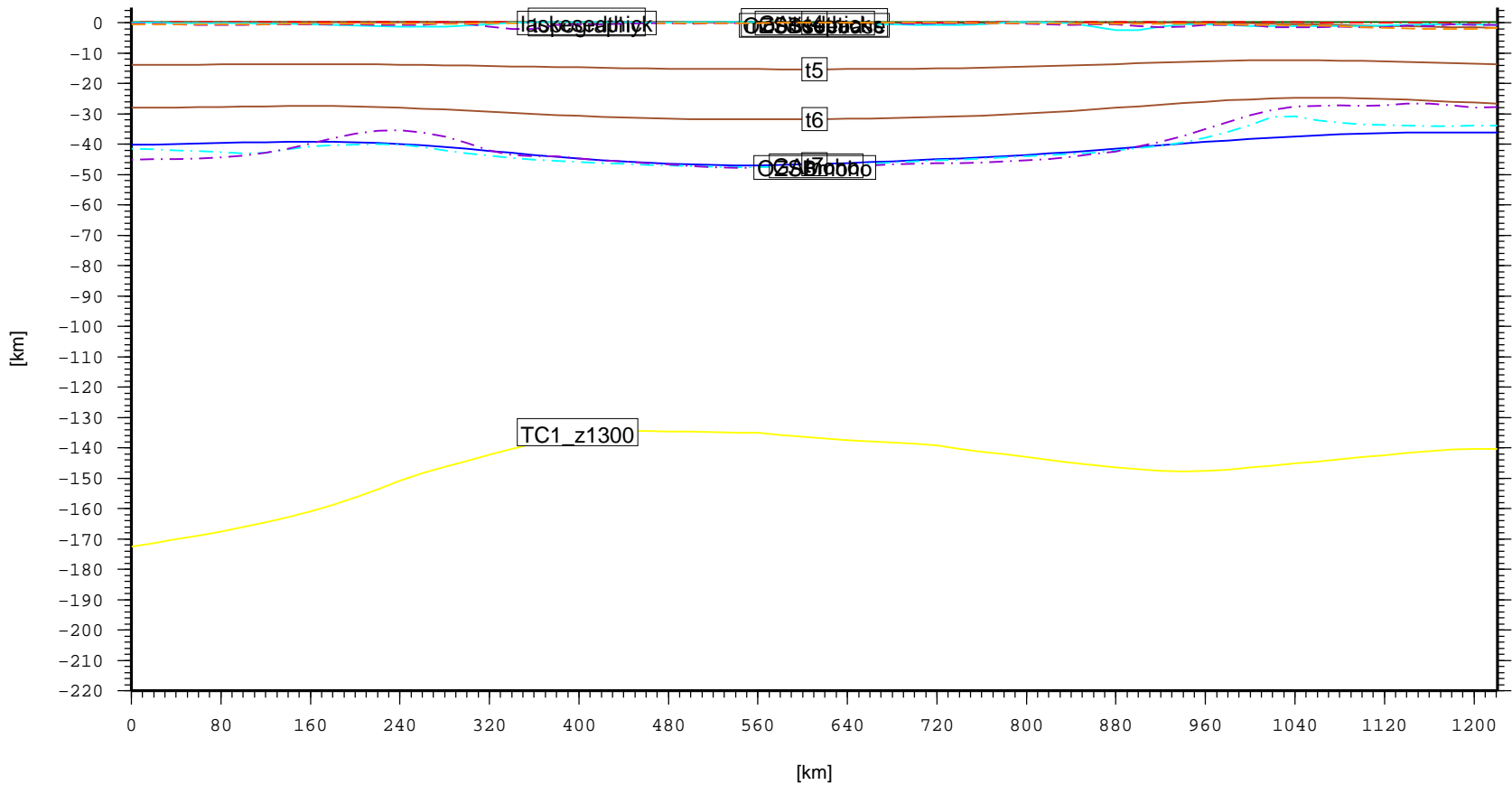
Cross section – AUS.GeorginaBasin (topo, laske sedthick, t4, t5, t6, t7)
