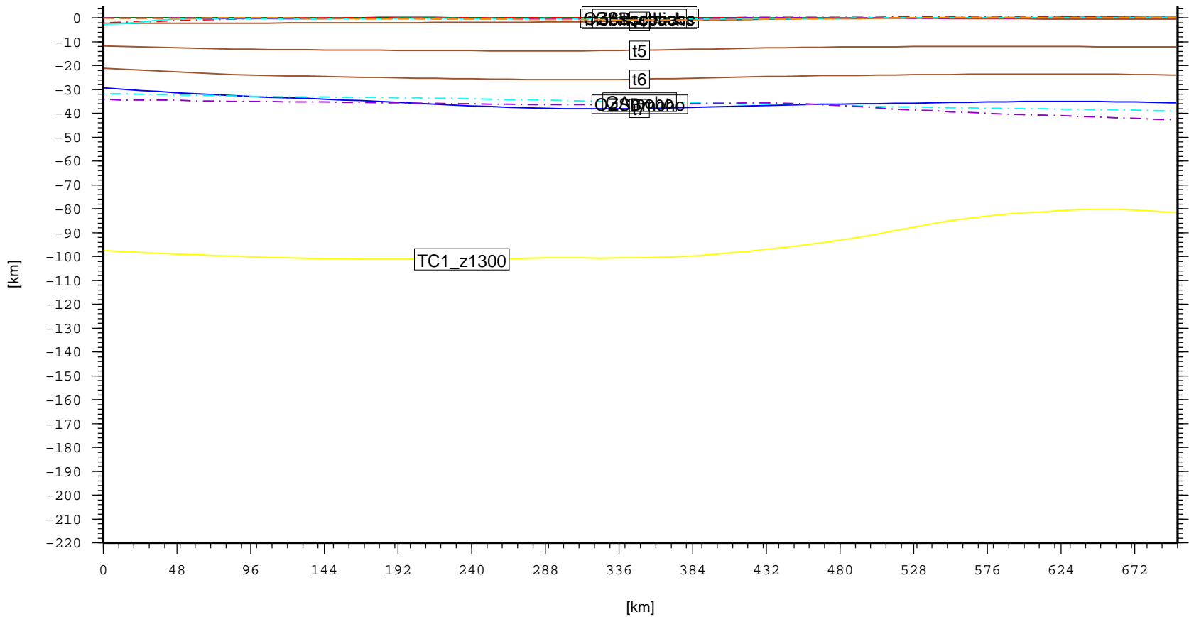
Cross section – AUS.MurrayBasin (topo, laske sedthick, t4, t5, t6, t7)
