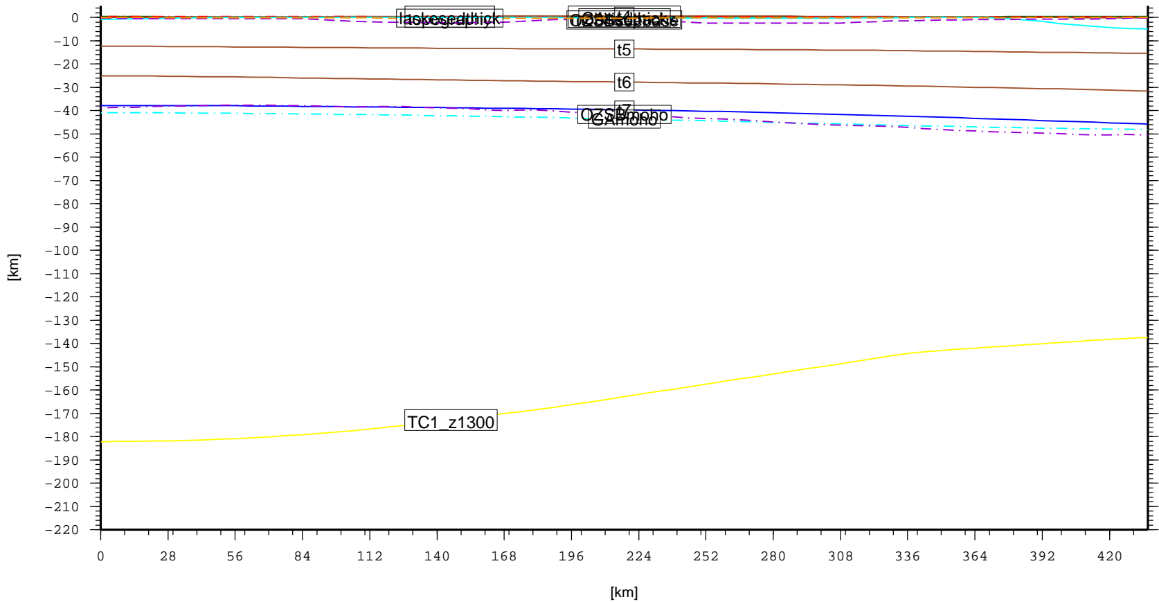
Cross section – AUS.WisoBasin (topo, laske sedthick, t4, t5, t6, t7)
