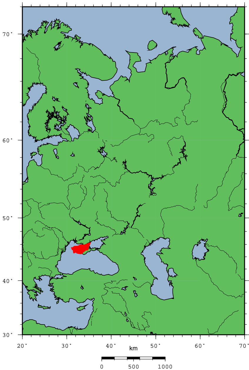
Location map CAS.NorthBlackSea–CrimeaBasin.
