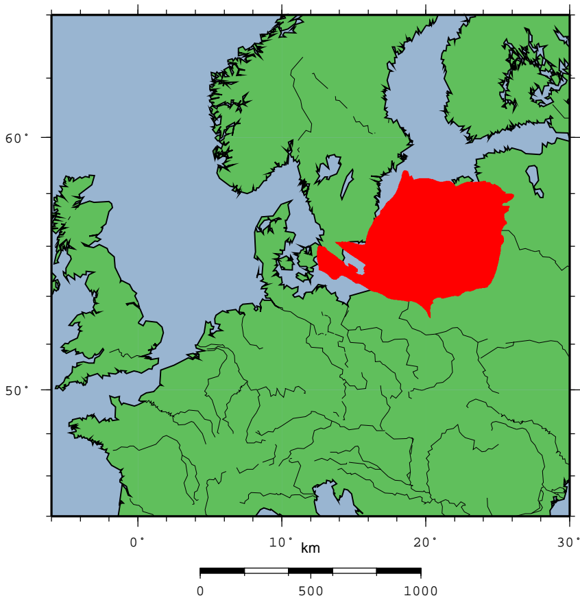
Location map EUR.BalticDepression.
