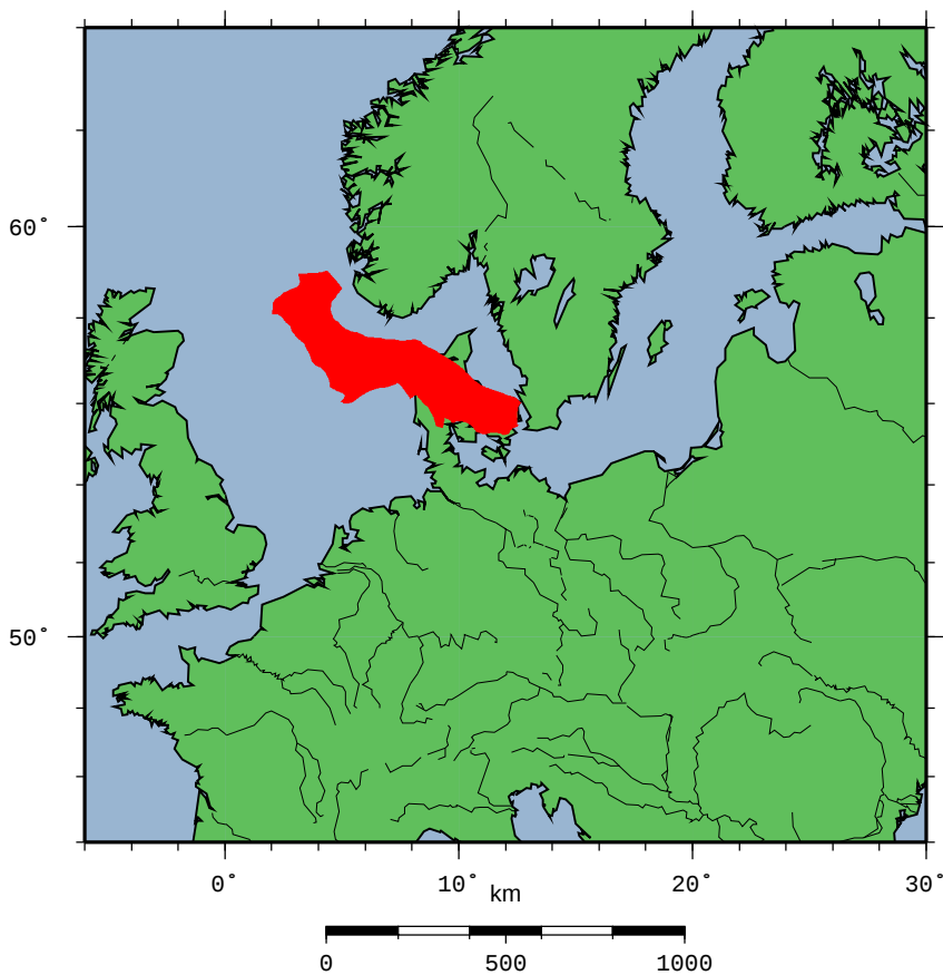
Location map EUR.Norwegian–DanishBasin.
