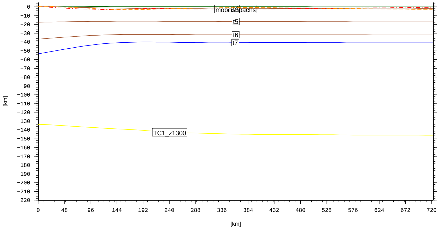
Cross section – SAM.CretaceousBasin (topo, laske sedthick, t4, t5, t6, t7)
