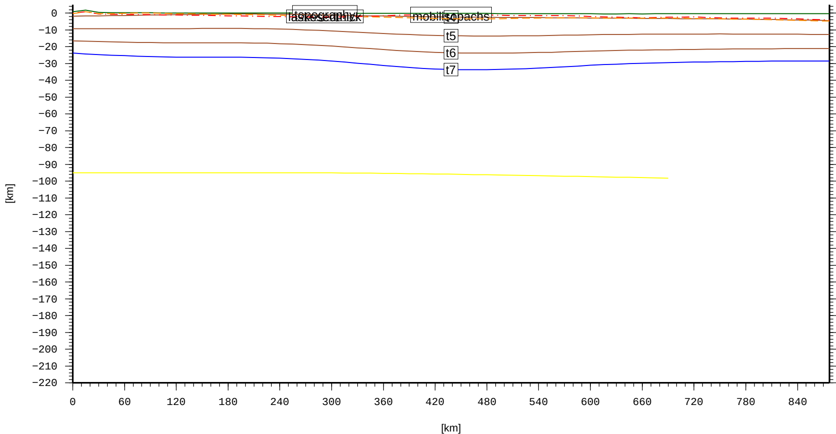
Cross section – SUN.NorthSumatraBasin (topo, laske sedthick, t4, t5, t6, t7)
