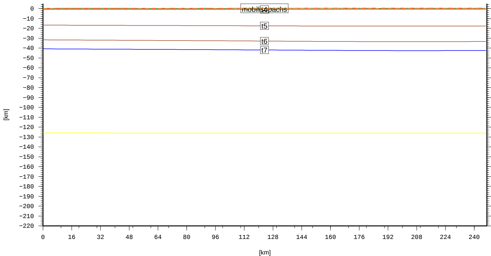
Cross section – SUN.PreahBasin (topo, laske sedthick, t4, t5, t6, t7)
