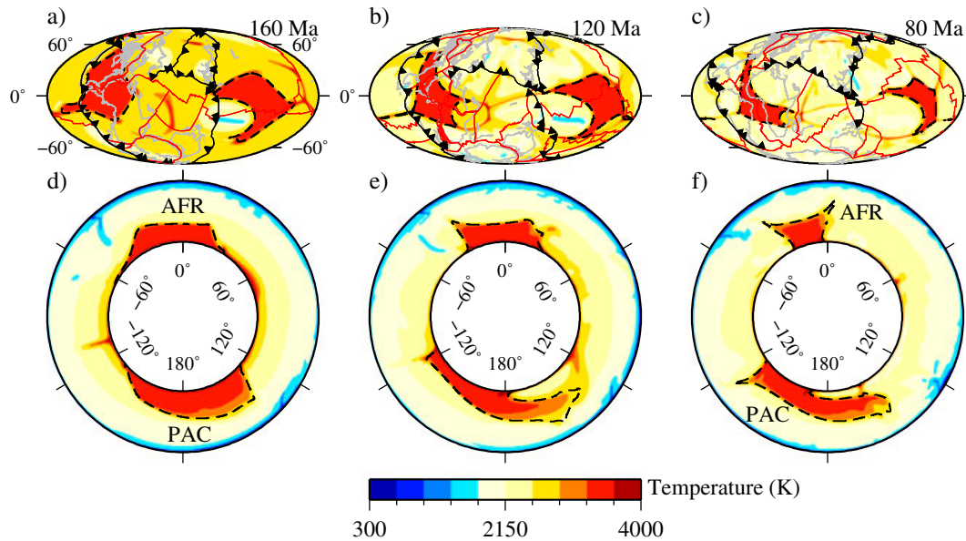
Figure 6. Model EX1 snapshots. (a, b, c) Temperature at 2600 km depth for 160, 120, and 80 Ma, respectively. (d, e, f) Equatorial annuli of temperature ( 0^\circ is the Prime Meridian) for Figures 6a, 6b, and 6c, respectively. For details, see Figure 4 caption.
