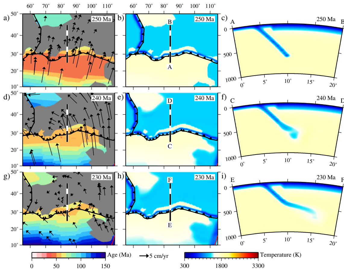
Figure 3. Progressive data assimilation example for the convergence of the Paleo-Tethys Ocean and Laurussia (Model BO6). Plate history and age of oceanic lithosphere model at (a) 250 Ma, (d) 240 Ma, and (g) 230 Ma. Temperature field at 110 km depth at (b) 250 Ma, (e) 240 Ma, and (h) 230 Ma. Cross section of slab (c) profile A–B, 250 Ma; (f) profile C–D, 240 Ma; and (i) profile E–F, 230 Ma. Ridges and transform faults are represented by red lines, and subduction zones are represented by black lines with sawteeth indicating polarity. Non-oceanic regions are dark gray.
