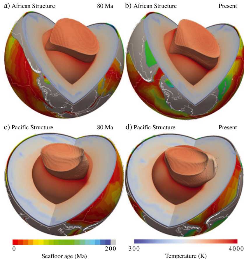
Figure 9. Three-dimensional view of the domes (Model EX5). African structure at (a) 80 Ma and (b) present. Pacific structure at (c) 80 Ma and (d) present. Ridges and transform faults are represented by red lines, and subduction zones are represented by black lines. Non-oceanic regions are dark gray, and reconstructed continents with present-day shorelines are shown in white.
