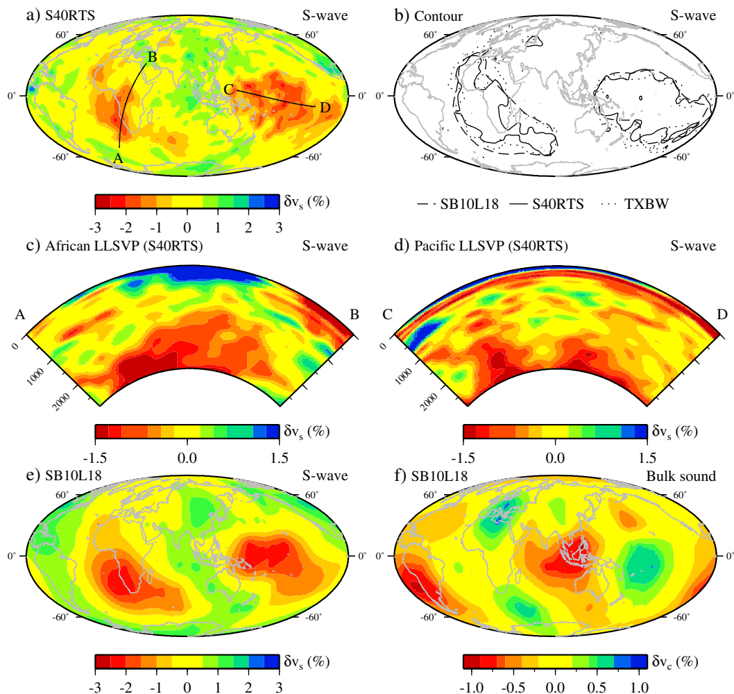
Figure 1. Seismic tomography data for the LLSVPs. (a) Shear velocity tomography model at 2800 km depth, S40RTS [Ritsema et al. , 2011]. (b) The -0.6\% shear velocity contours from several S-wave tomography models (SB10L18, S40RTS, TXBW [Grand, 2002]) at 2800 km depth show their consistency. (c, d) Cross section through the African and Pacific LLSVPs, respectively. The color scale is saturated to highlight mid-mantle structure. Locations of cross sections are marked on Figure 1a. (e) Shear velocity tomography model at 2800 km depth, SB10L18 [Masters et al. , 2000]. (f) Bulk sound speed from SB10L18 [Masters et al. , 2000] at 2800 km depth. Note approximate anticorrelation with shear velocity in Figure 1e.
