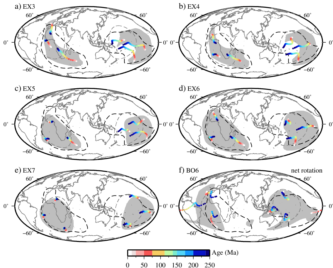
Figure 8. Motion and deformation of the domes at 2600 km depth, (a) EX3, (b) EX4, (c) EX5, (d) EX6, (e) EX7, and (f) BO6. The gray-shaded region shows the domes at present day, and the gray dashes contour the initial position of the domes at 250 Ma. Black dashes delineate the -0.6\% S -wave contour from SB10L18, and continent outlines are shown in solid dark gray. Color-coded dots track the movement of points located within the domes at the CMB from 250 Ma to present day.
