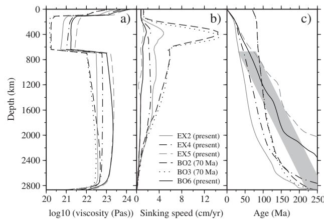
Figure 10. Radial profiles for (a) viscosity, (b) slab sinking speed, and (c) approximate age of subducted material versus depth for EX2, EX4, EX5, and BO6 at present day and for BO2 and BO3 at 70 Ma. For depths >2000 km, the average viscosity may be reduced by the hot domes. Sinking speed is determined from positive density anomalies that are greater than 25% of the maximum positive density anomaly at each depth and time [e.g., Steinberger and Torsvik, 2010]. We set the velocities for depths <128 km to the value at 128 km depth because they are influenced by data assimilation. The age-depth relation is computed by integrating the time- and depth-dependent slab sinking speed, and the gray-shaded region shows a geological estimate [van der Meer et al. , 2010].
