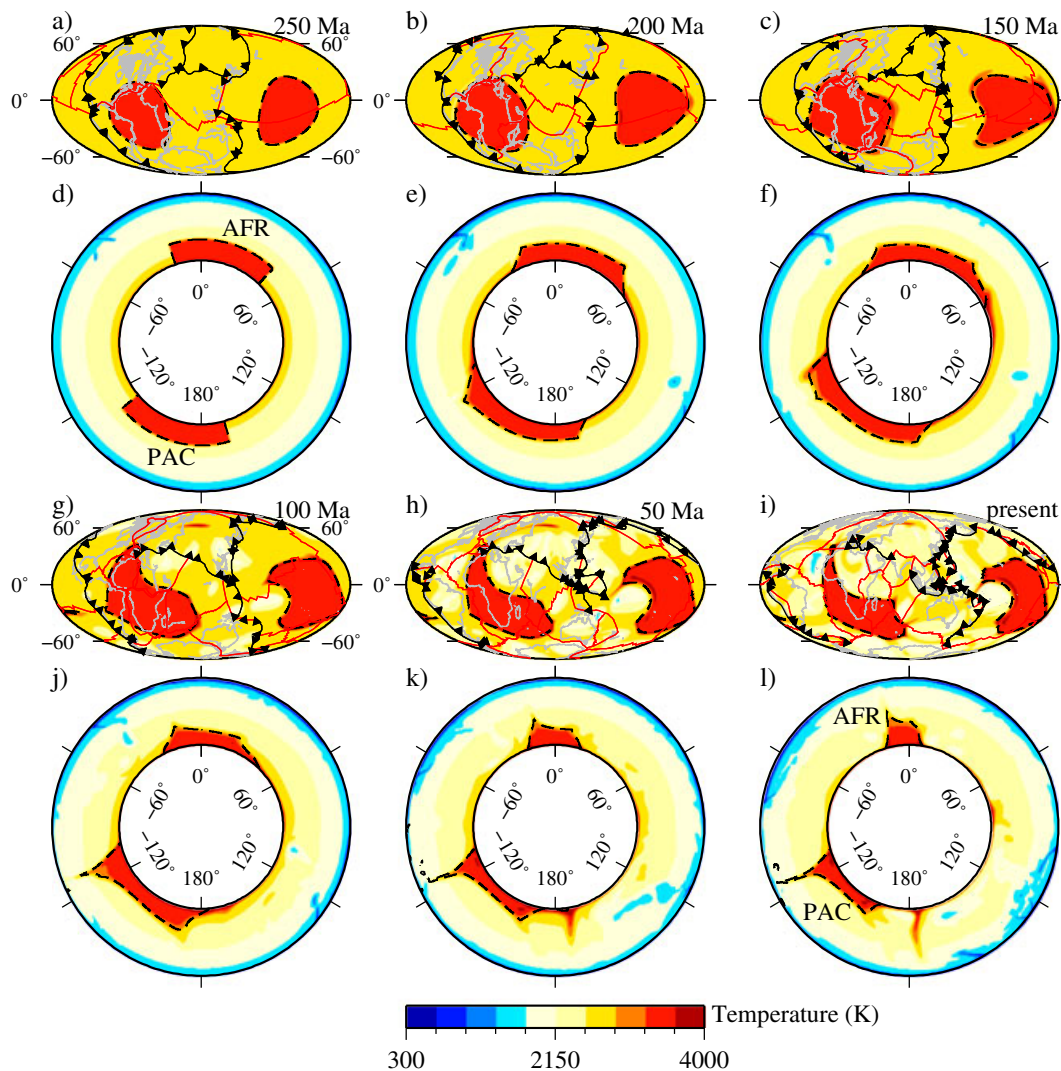
Figure 4. Reference model (EX4) snapshots. (a, b, c, g, h, i) Temperature at 2600 km depth for 250, 200, 150, 100, and 50 Ma and present day, respectively. The compositionally distinct material is contoured with black dashed lines. Ridges and transform faults are represented by red lines, and subduction zones are represented by black lines with saw-teeth indicating polarity. Reconstructed continent outlines are shown in light gray. (d, e, f, j, k, l) Equatorial annuli of temperature (0° is the Prime Meridian) for Figures 4a, 4b, 4c, 4g, 4h, and 4i, respectively. “AFR” and “PAC” identify the domes.
