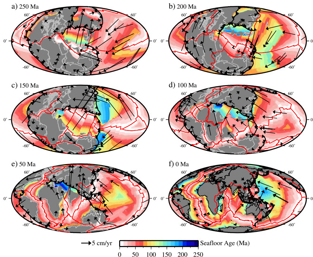
Figure 2. Snapshots of the plate tectonic reconstruction extended from Seton et al. [2012]. (a) 250 Ma, (b) 200 Ma, (c) 150 Ma, (d) 100 Ma, (e) 50 Ma, and (f) present day. Ridges and transform faults are represented by red lines, and subduction zones are represented by black lines with sawteeth indicating polarity. Non-oceanic regions are dark gray, and reconstructed continents with present-day shorelines are shown in light gray (except black for the present day).
