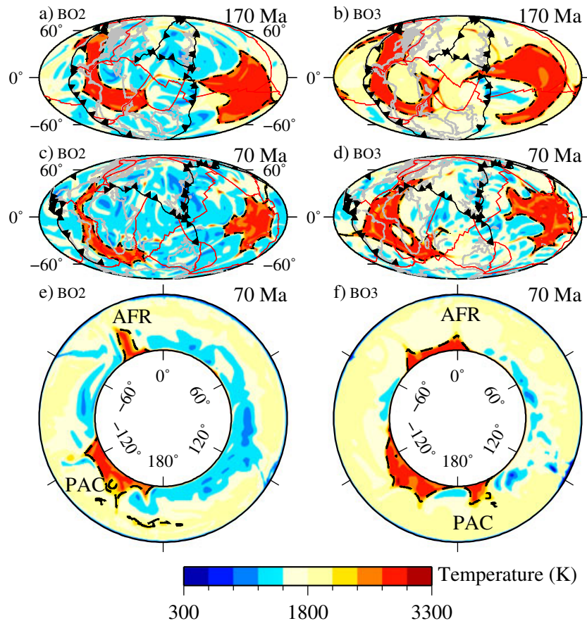
Figure 7. BO2 (with assimilation) and BO3 (kinematic only) snapshots. Temperature at 2600 km depth for (a, c) BO2 at 170 and 70 Ma, respectively. (b, d) BO3 at 170 and 70 Ma, respectively. (e, f) Equatorial annuli of temperature ( 0^\circ is the Prime Meridian) for Figures 7c and 7d, respectively. For details, see Figure 4 caption.
