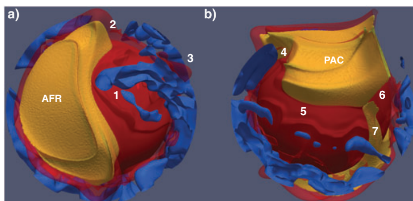
Figure 5. Three-dimensional view of the domes, plumes, and slabs at 90 Ma (Model EX4). The 2500 K isosurface is colored red and is transparent so that the (a) African (“AFR”) and (b) Pacific (“PAC”) domes (colored yellow) are visible on the CMB. Slabs are colored blue, and the upper thermal boundary layer has been removed for clarity. See text for discussion of the labeled regions (1–7).
