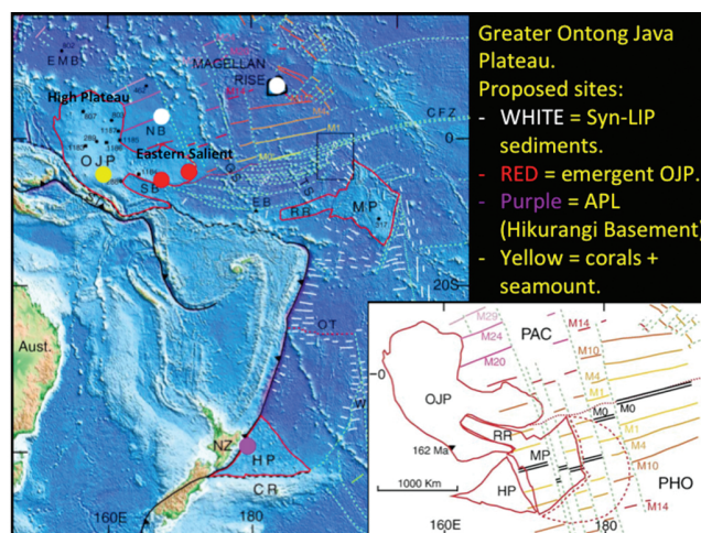
Figure 2. Present configuration of large igneous provinces (LIPs) in the SW Pacific (outlined in red) with proposed drilling sites. The inset shows reconfiguration of the Greater Ontong Java Plateau (OJP) suggesting the Ontong Java and Hikurangi (HP) plateaus and the Manihiki Plateau (MP) all formed during a single event adapted from Taylor (2006). Note: Robbie Ridge (RR), Ellis Basin (EB), East Mariana Basin (EMB), Nauru Basin (NB), Clipperton Fracture Zone (CFZ), Osborn Trough (OT) and Chatham Rise (CR) are also shown. The inset shows a reconstruction at ~ 125 Ma prior to breakup and before Pacific (PAC) – Phoenix (PHO) spreading (from Taylor, 2006).
